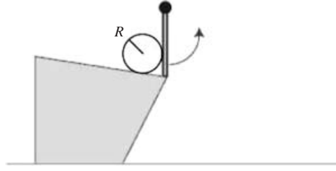
FIGURE 7. Our device for varying the size of the bouncing drop: a volume of water (radius R ) is deposited on a slightly inclined plate. When the gate is opened, the drop falls and bounces on the plate below. All the elements are made of steel and heated, so that the drop is everywhere in a Leidenfrost situation.
