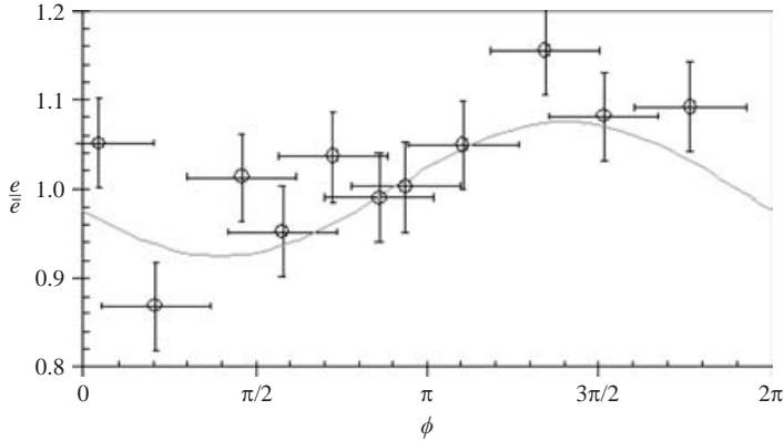
FIGURE 17. Restitution coefficient of a drop bouncing off a hot plate as a function of its phase at impact (defined in figure 15). The restitution coefficient is normalized by its mean value at a given impact velocity. Each datum corresponds to at least five experiments, and the corresponding error bars are indicated.
