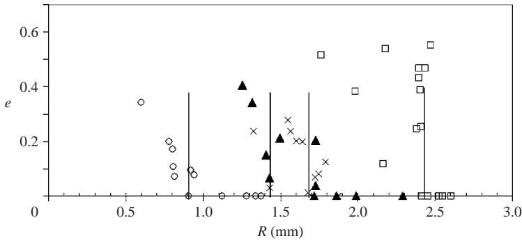
FIGURE 8. Restitution coefficient of the shock for a drop of varying radius R falling from a given height H = 1 cm, as a function of R for different liquids (○, liquid nitrogen; ▲, ethanol; ×, acetone; □, water). In each case, an abrupt decrease is observed around a critical radius R_c marked with a vertical line.
