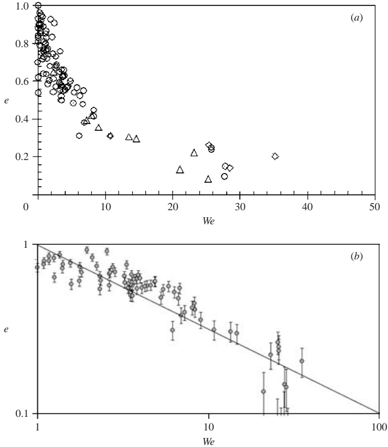
FIGURE 4. Restitution coefficient e for Leidenfrost drops ( \circ , water; \triangle , acetone; \diamond , ethanol; \square , nitrogen) bouncing on plates at temperature much larger than the boiling point of the liquid. The drop radii vary between 0.8 and 2 mm, and the impact velocities between 0.02 and 1 m s -1 . (a) It is found that the data collapse on a single curve, if they are plotted as a function of the Weber number We defined in (1). The elasticity strongly decreases with We . (b) If the same data are displayed in a log-log plot, e is observed to decrease as We^{-1/2} drawn with a line. Writing e = \alpha We^{-1/2} , we find from the fit a numerical coefficient \alpha = 1.0 \pm 0.1 .
