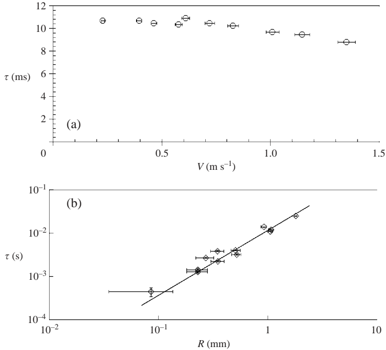
FIGURE 2. Contact time \tau of a drop bouncing on plate heated at 280^\circ\text{C} . (a) \tau is plotted as a function of the impact velocity V (for a fixed drop radius R = 1.06 mm), and found to be quite insensitive to V (multiplying V by a factor of about 7 makes \tau decrease by only 15%). (b) \tau is observed (in a log-log plot) to increase rapidly with the drop radius R , as R^{3/2} (solid line). Writing \tau = \alpha (\rho R^3 / \gamma)^{1/2} , we deduce from the fit a numerical coefficient \alpha = 2.65 \pm 0.20 .
